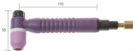
WON150A 空冷可弯曲长焊枪 WT150FL 5-39 WON150A 공냉 후렉시블 롱 토치 WT150FL 5-39
