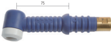
WON400A 空冷可弯曲焊枪 WT400F 40-104 WON400A 공냉 후렉시블 토치 WT400F 40-104
