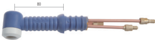
WON400A 水冷可弯曲焊枪 WT400FW 40-104-2 WON400A 수냉 후렉시블 토치 WT400FW 40-104-2
