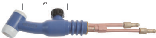
WON350A 水冷带阀可弯曲焊枪 WT18FVW 6-78-2 WON350A 수냉 밸브 후렉시블 토치 WT18FVW 6-78-2
